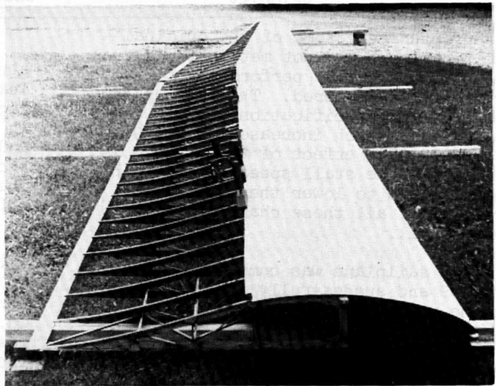
FIGURE 2. WING SPAR CONSTRUCTION
