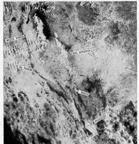
Figure 7. Enhanced Infrared VHRR companion to Fig. 6.
