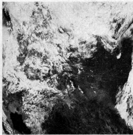
Figure 5. This half mile resolution visual channel image of the south-western portion of the United States was obtained from the NOAA-2 Very High Resolution Radiometer (VHRR) near 8:40 AM local time on March 28, 1973. The region covered extends from Salt Lake to the California Gulf in the west and from Mid-Kansas to the lower Rio Grande along the eastern edge.
