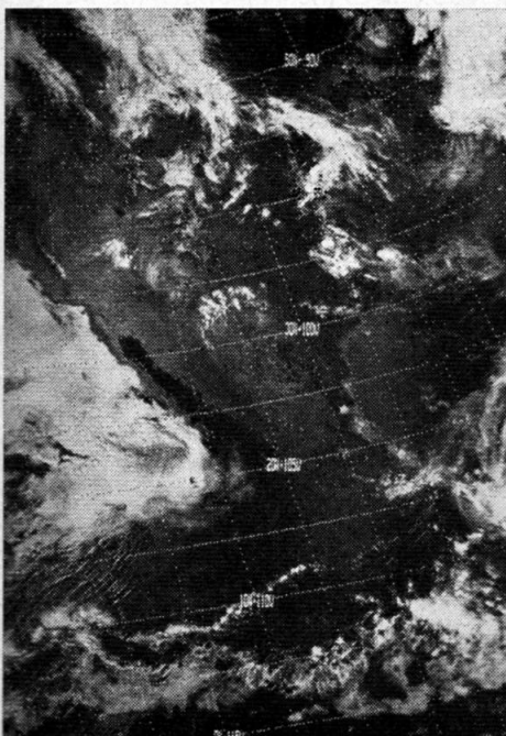
Figure 1. Visual channel image from the NOAA-2 Scanning Radiometer (SR) near 9 AM local time on May 21, 1973. Earth locator lines and labels are implanted in the image as the digital samples are geometrically altered to an approximate equal area projection.
