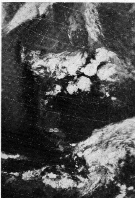
Figure 2. Infrared view obtained from the NOAA-2 SR near 9 PM local time on May 22, 1973.
