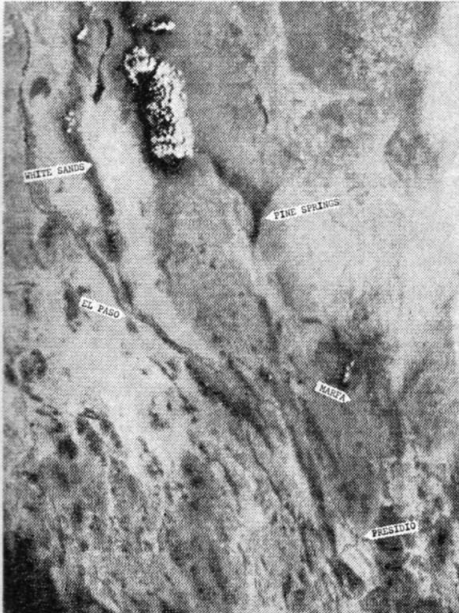
Figure 8. Enhanced visual channel VHRR image obtained on April 12, 1973 in approximately the same area as shown in Figs. 6 and 7.
