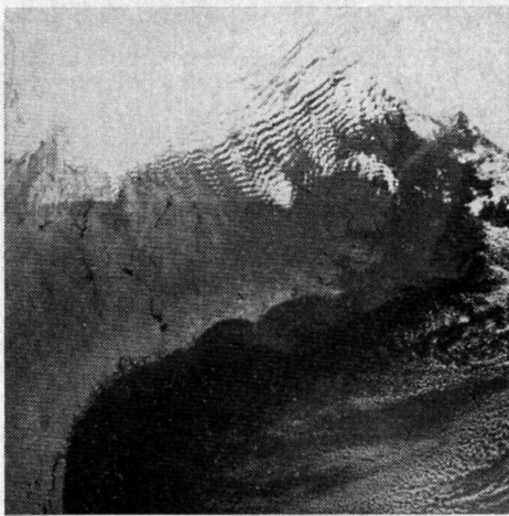
Figure 4. Infrared view of Appalachian wave clouds obtained from the NOAA-2 Very High Resolution Radiometer (VHRR) near 9 PM on March 12, 1973.
