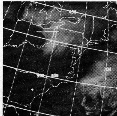
Figure 3. Appalachian wave clouds as seen by the ESSA-9 vidicon camera near 3 PM on February 21, 1970.
