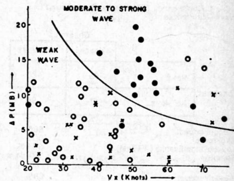
Figure 1. Verification of Harrison's Lee Wave Prediction Nomogram. Open circles indicate reported weak cases. Solid circles indicate strong wave cases. \Delta P : Grand Junction Sea Level Pressure minus Denver Sea Level Pressure. V_x : Maximum winds 10,000 to 20,000 ft ASL. (From Harrison, 1957)
