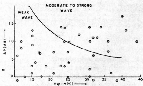
Figure 5. Harrison Nomogram With SWP and CLWP Data. Lee waves were observed in all cases. For CLWP cases, \Delta P is the sea level pressure difference between Grand Junction and Denver, Colorado. \Delta P for SWP is the difference between the sea level pressures at Fresno, California and Tonopah, Nevada plus 2 mb. V_{xp} is the maximum wind component perpendicular to the ridgeline between 10,000 and 20,000 feet.
