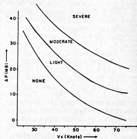
Figure 2. GWC Wave Prediction Nomogram. The layer through which the maximum wind is computed depends on the height of the mountain. Intensities refer to turbulence associated with the lee wave (redrawn from Burnett, 1970).
