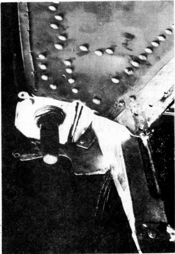
Figure 5. Fatigue Failure at the Rear Wing Attachment Bolt.
