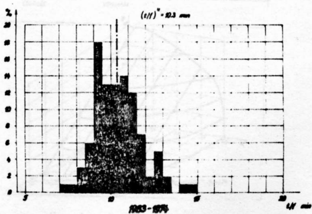
Figure 1. Average Flying Time Histogram.
