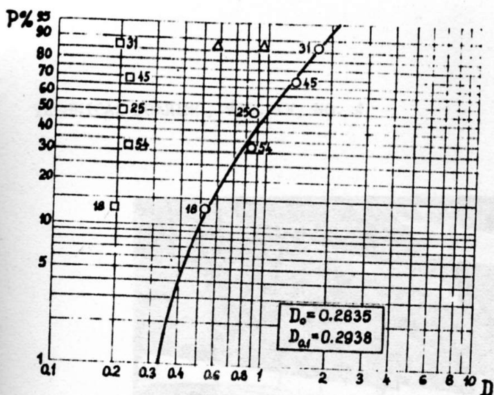
Figure 8. Fatigue Life Distribution in D
