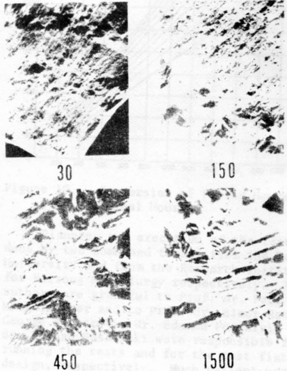
Figure 6. Scanning Electron Micrograph of the Spar Boom Fracture.
