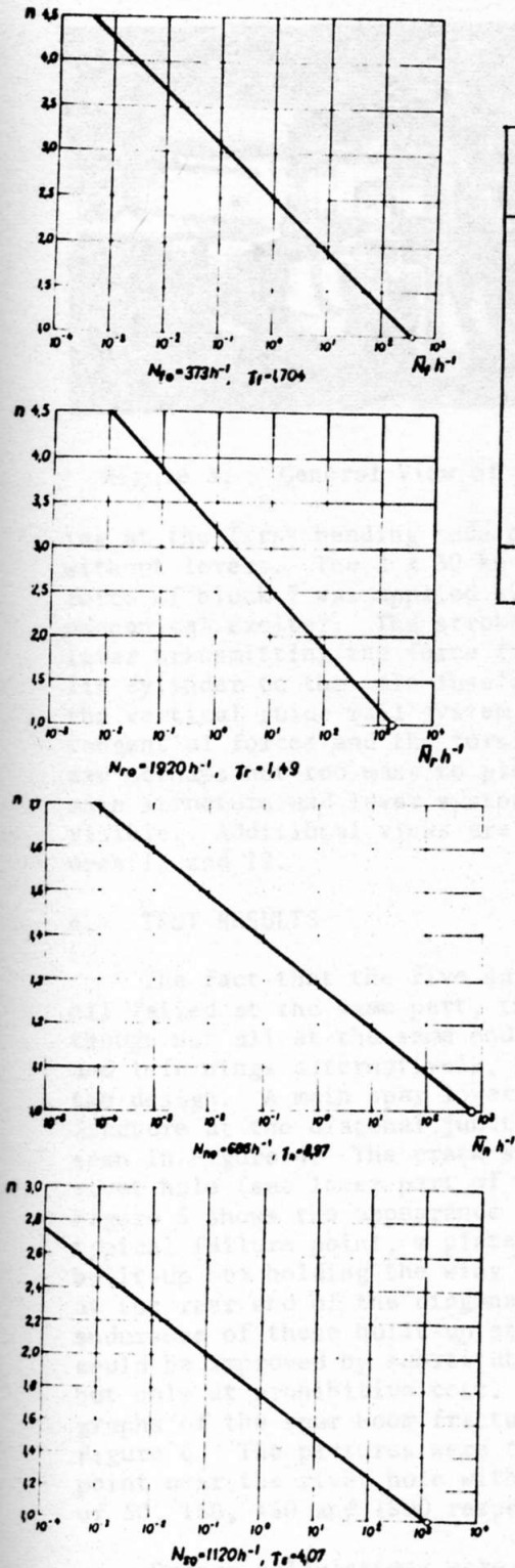
Figure 2a. Service Load Spectra: Start-landing, Aero Tow, Calm Air Flying, Gliding between Thermals.
