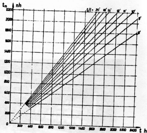
Figure 10. Conversion of Flying Hours into Normal Hours.
