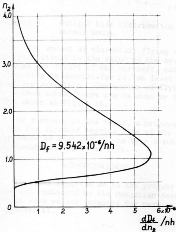
Figure 7. Damage Curve for Start and Landing.
