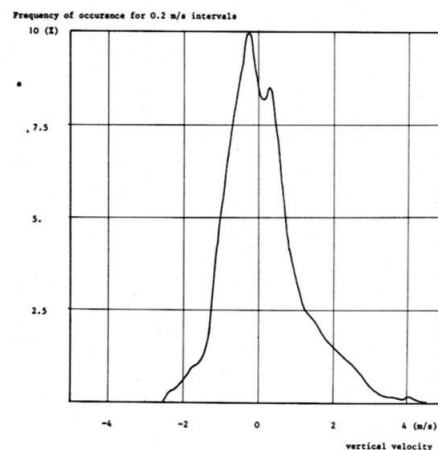
Figure 1: Frequency of occurrence of vertical velocity intervals Meppen, 25th of April, 1974, 16.02–16.18 in 300 m above ground (standard deviation \sigma_w = 1.02 m/s, skewness = 0.74, kurtosis = 0.82).
