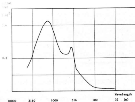
Figure 4: Spectral energy of vertical velocity (m/s) 2 Meppen, 25th of April, 16.02–16.18 in 300 m above ground.
