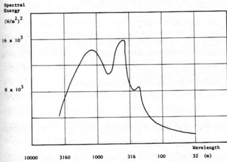
Figure 5: Spectral energy of vertical flux of sensible heat (W/m 2 ) 2 Meppen, 25th of April 1974, 16.02–16.18 in 300 m above ground.
