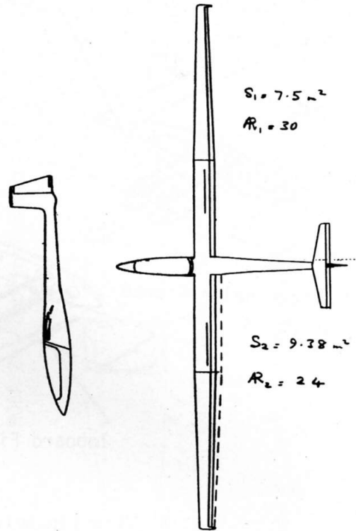
Fig. 7 MOBA 3: "VIRAGO" 15M Variable Geometry Sailplane
