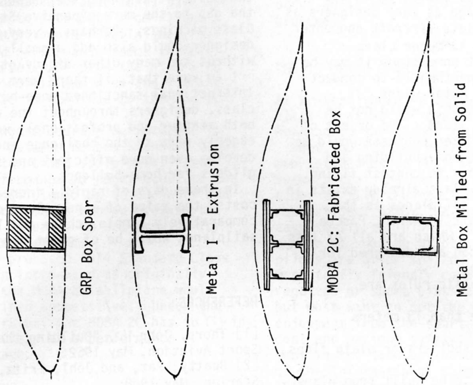
Fig. 2 Typical Spar Boom Locations
