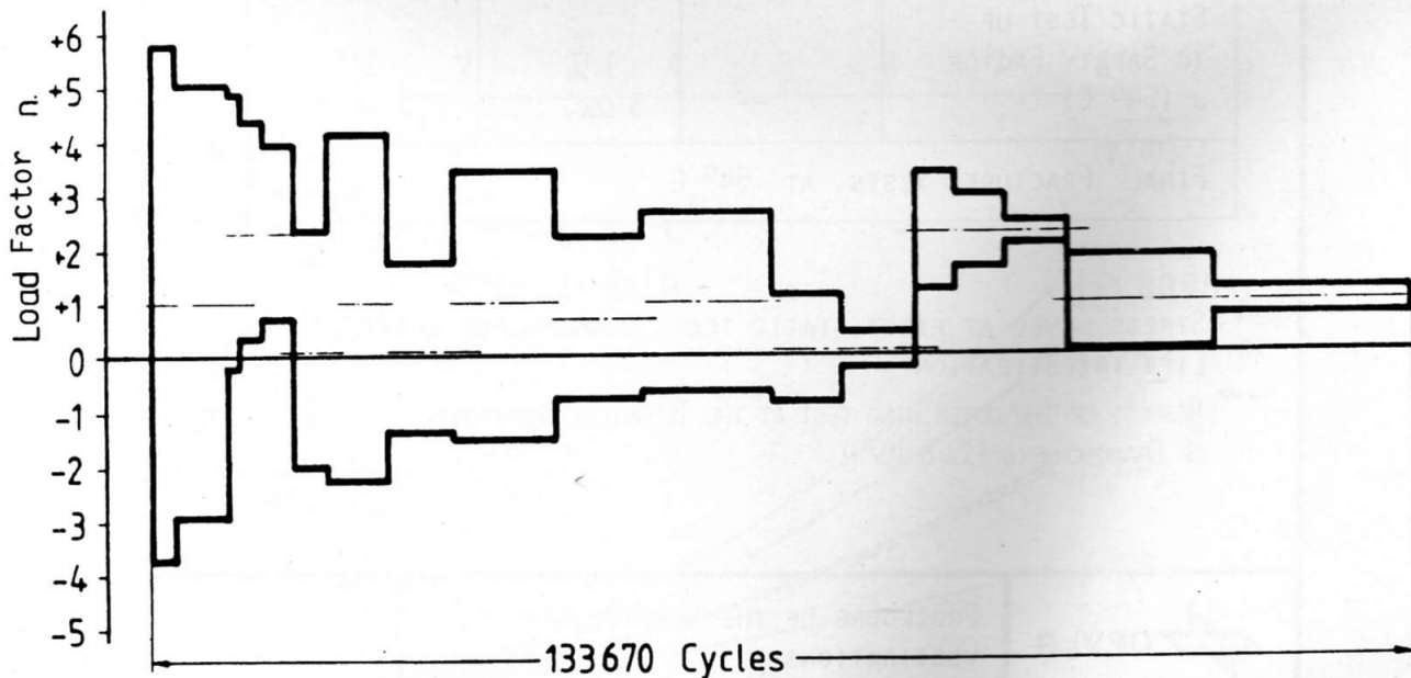
Fig.11 Splitting and Rearrangement of the Service Life Program for 24h - Cycle
