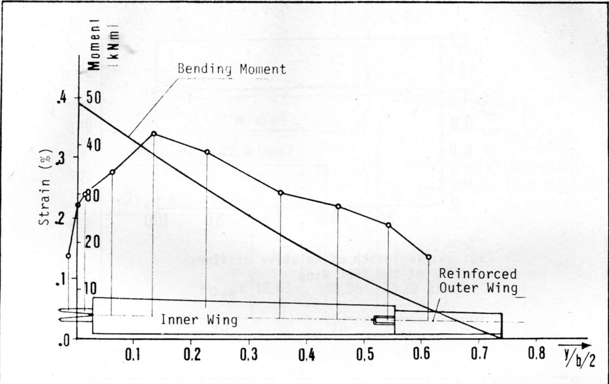
DFVLR Strain Distribution in Upper Spar Cap for Bending Moment Corresponding to Design Load Fig. 13
