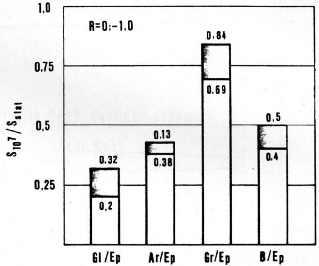
Fig.2 Fatigue limits of UD composites [4]
