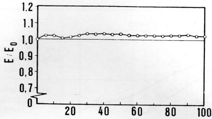
Fig. 15: Variation of Relative Stiffness of the CFRP Wing
