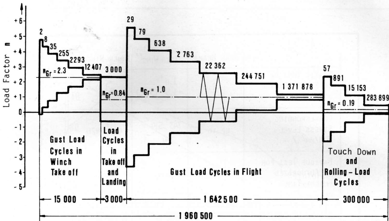
Fig.10 Service Life Program corresponding to 1000 Authorized Flight Hours
