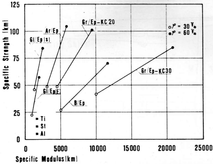
Fig.1 Specific Strength vs. Specific Modulus UD-Composites, Ref. [1]
