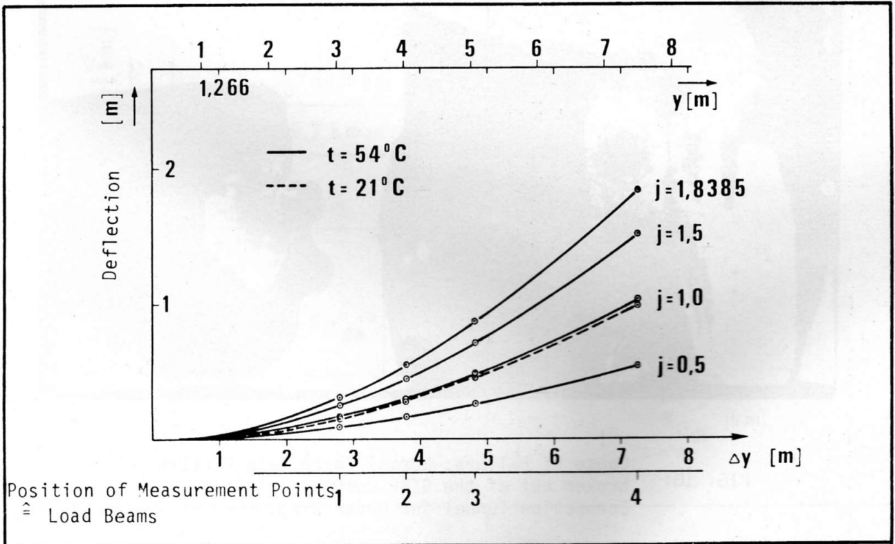
DFVLR Bending Line of CFRP Wing for j = 0.5, 1.0, 1.5, \text{ and } 1.8385 (Failure) Fig. 14
