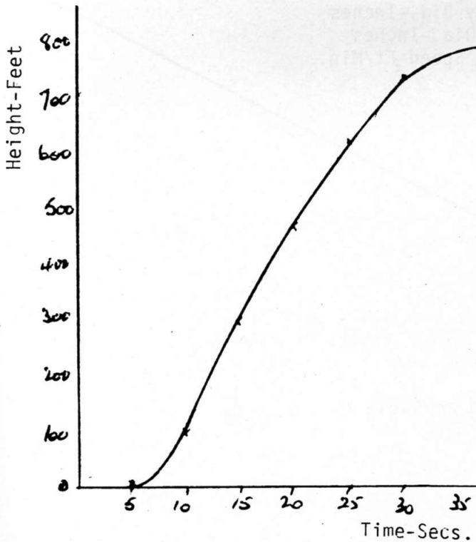
Fig. 3. Height/Time For Winch Launch
