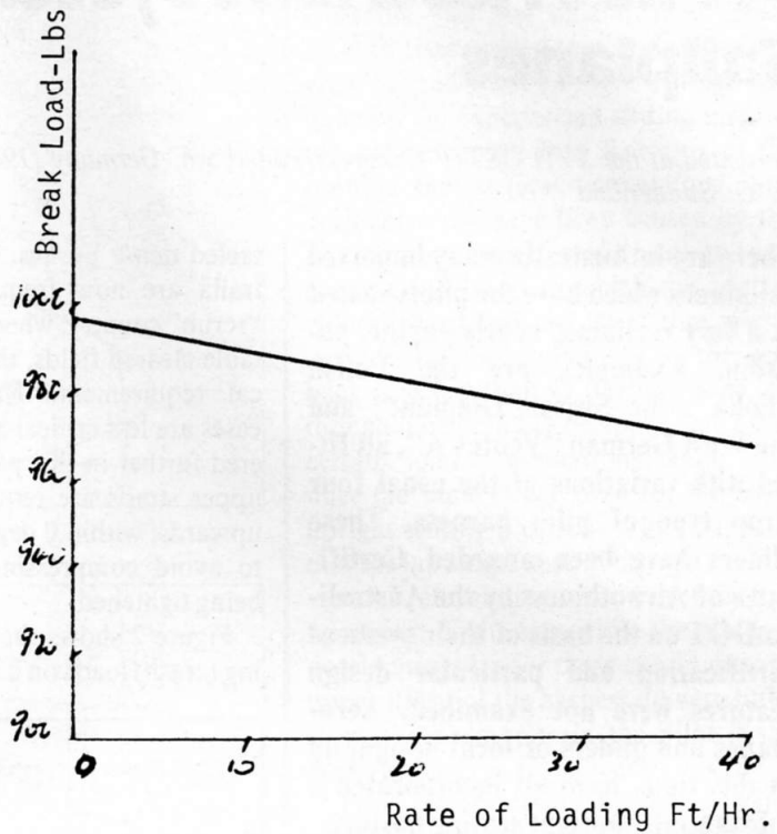
Fig. 9. Break Load. Variation with Rate of Loading. 3-Hole Plate Weak Link.
