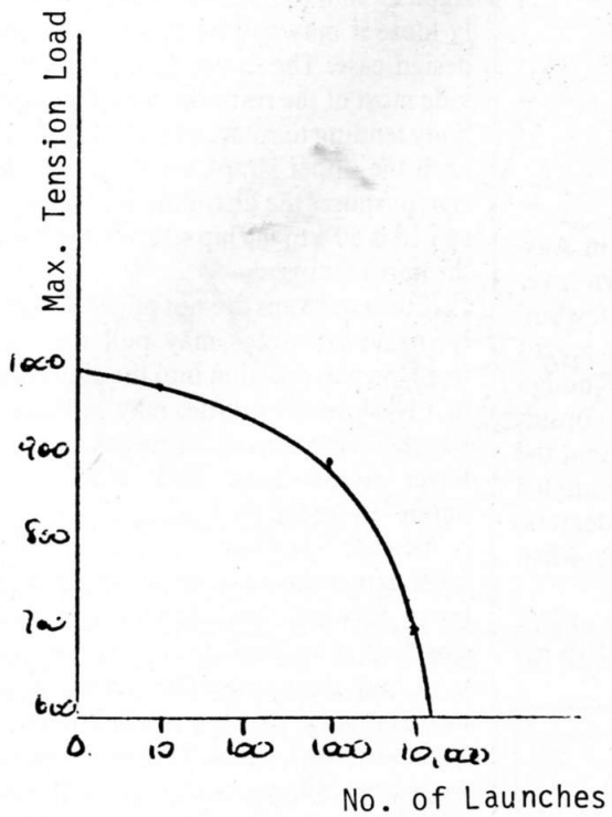
Fig. 8. 3-Hole Plate. Variation of Break Hold With Usage.
