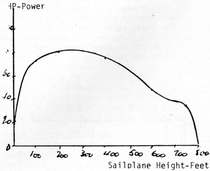
Fig. 5. BHP & Height Sailplane AOW AOW = 526 lbs; 826 lbs
