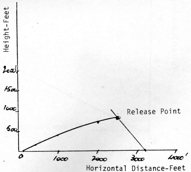
Fig. 4. Vertical & Horizontal Height Relation
