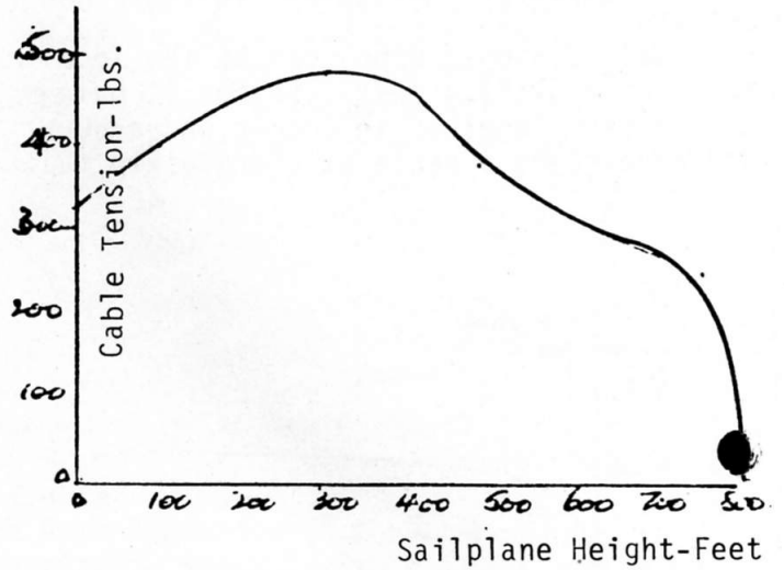
Fig. 6. Cable Tension & Height
