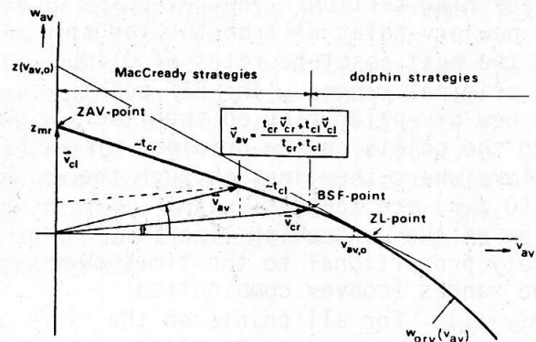
Fig. 6: The orv-polar for the range and atmospheric vertical velocity distribution of Fig. 5
