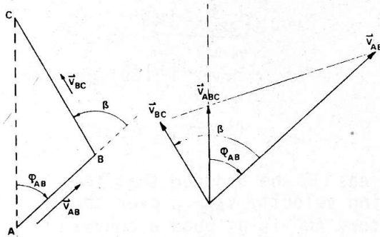
Fig. 14: The resulting velocity v_{ABC} over the broken trajectory A-B-C and the fly-off angle \beta
