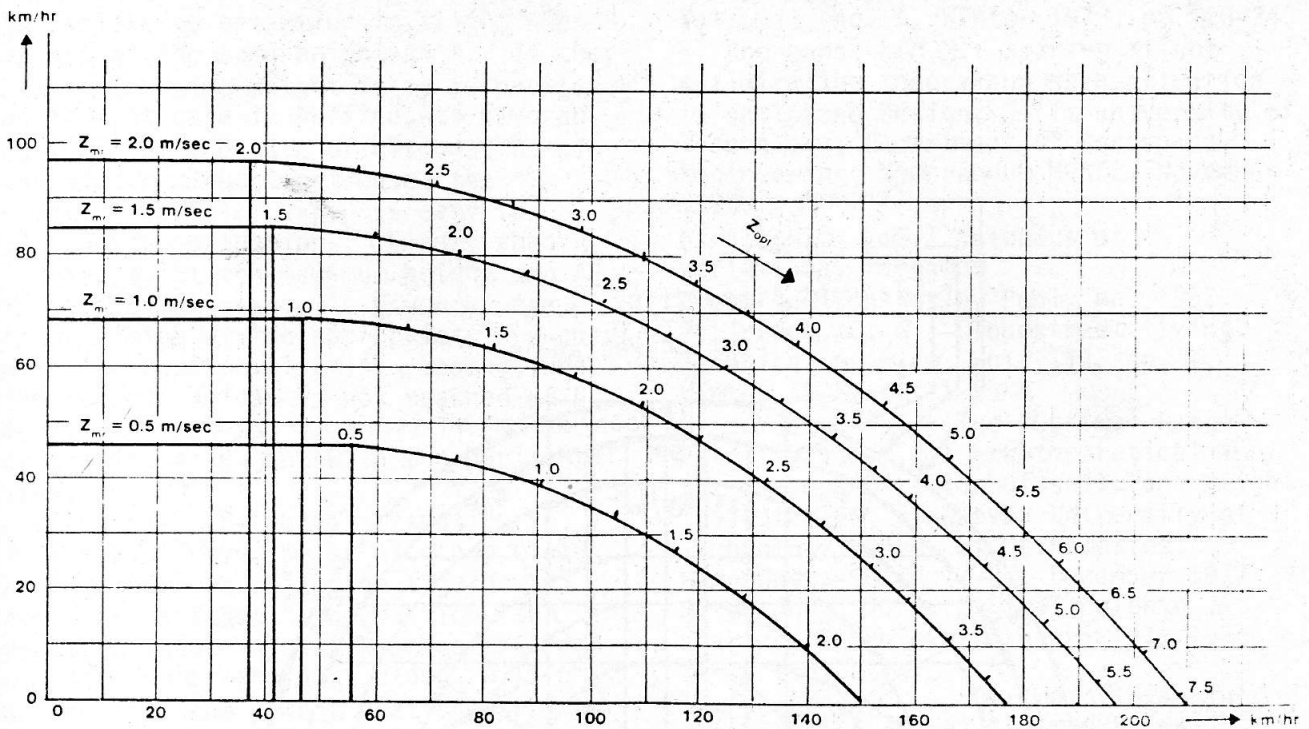
Fig. 28: Optimal-velocity or orv-curves for an LS-3 sailplane with a wing loading of 45 kg/m 2
