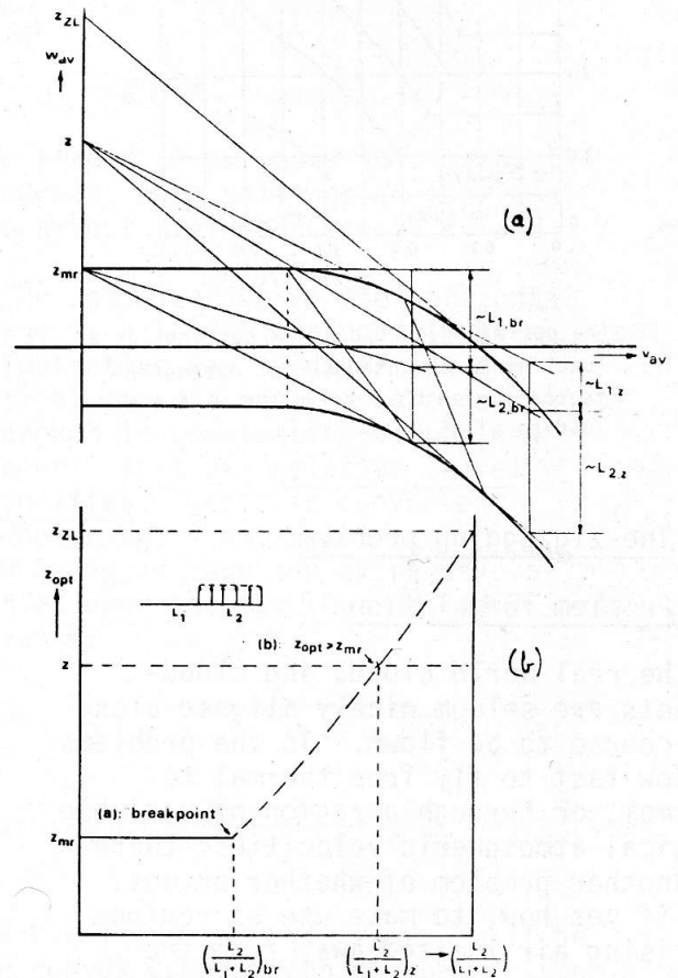
Fig. 11: Graphical construction of a plot of optimal MacCready ring settings as a function of the cloudstreet extension ratio L_2/(L_1 + L_2)
