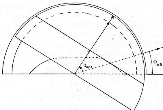
Fig. 32: Principle of operation of the zigzag computer
