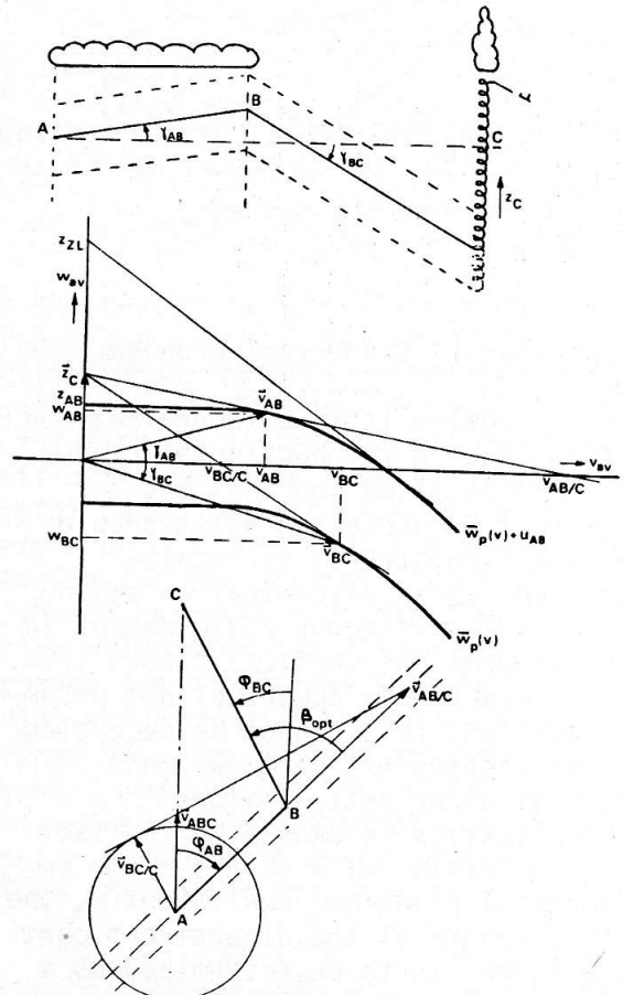
Fig. 21: The graphical determination of the optimal fly-off angle \beta_{opt} in case of a single cloudstreet and z_C \geq z_{AB} (cf. Fig. 20a,b,c)
