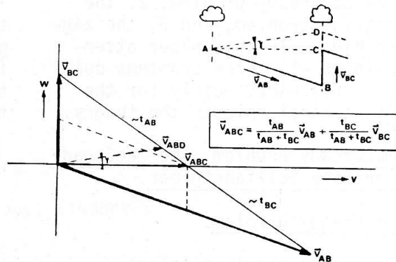
Fig. 3: The convex combination properties
