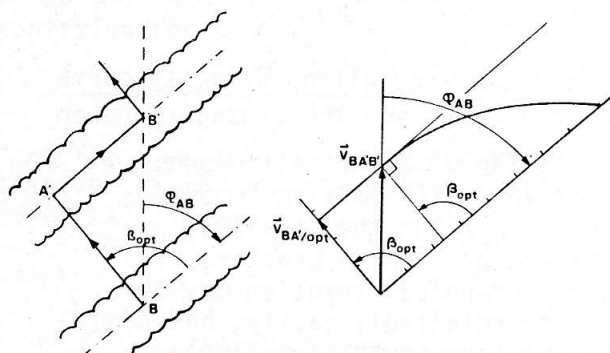
Fig. 29: Example of the use of the orv-curve for the determination of the optimal fly-off angle and the optimal MacCready ring setting in case of parallel cloudstreets
